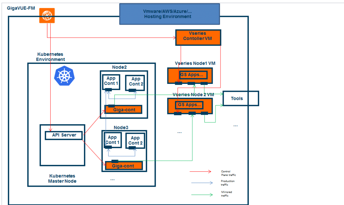
Figure 1: GigaVUE Cloud Components for Kubernetes using G-vTAP Containers
